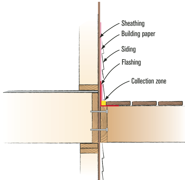
Figure 4. Although it's common practice to bring an L-shaped flashing down the wall and kick it out over the ledger, the resulting pocket can collect debris, and rot both the decking and the siding above.
