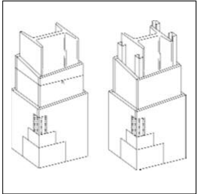
Figure 6 Column Protection - Gypsum Board or Veneer Base
