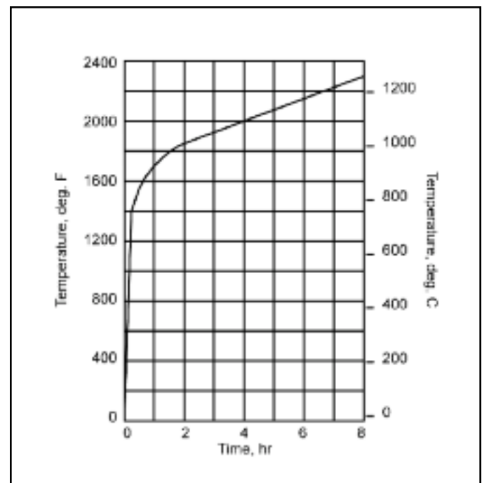
Figure 2 Standard Time-Temperature Curve (ASTM E 119)
