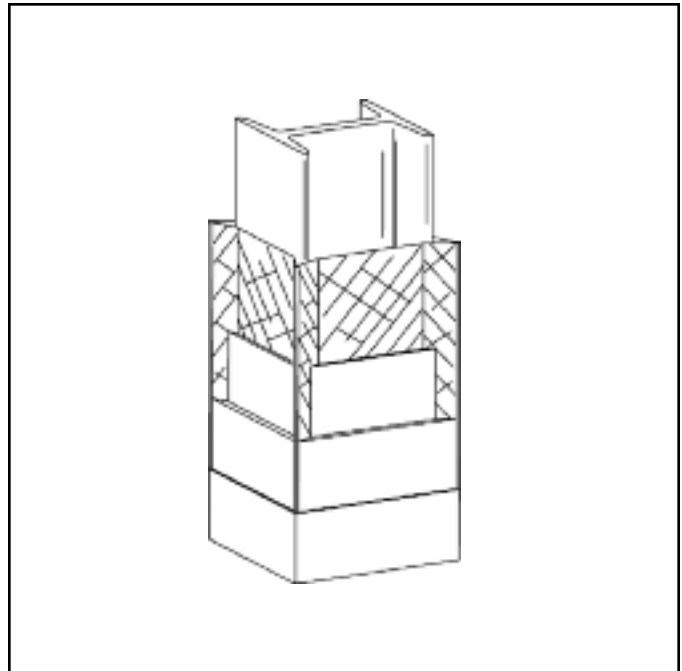
Figure 7 Column Protection - Metal Lath and Plaster
