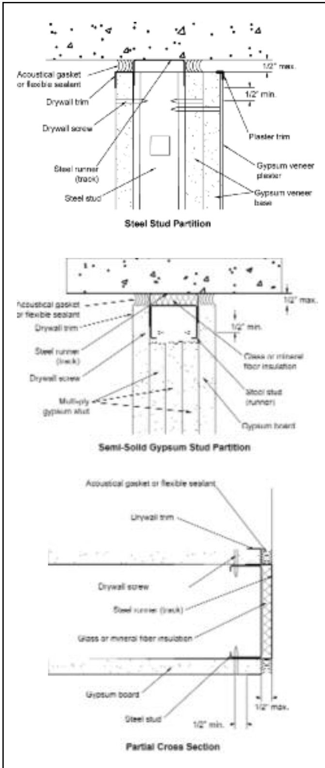
Figure 8 Perimeter Relief Details (FM 16738.69, 6/18/69; UL R4024-7-8, 6/23/66)
