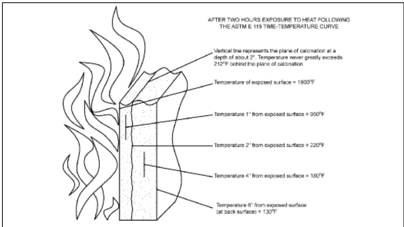
Figure 1 How Gypsum Retards Heat Transmission
