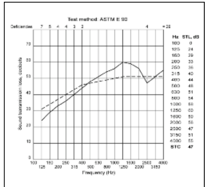
Figure 12 STL Curve
