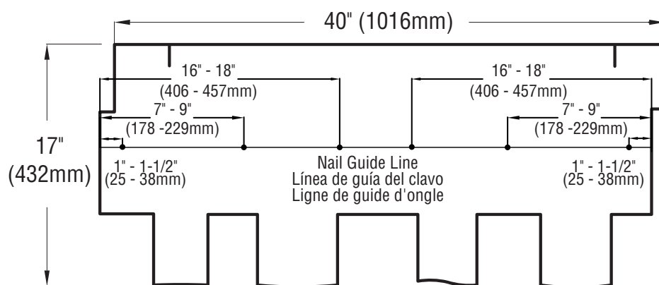
ENHANCED NAILING PATTERN - six nails per shingle*
